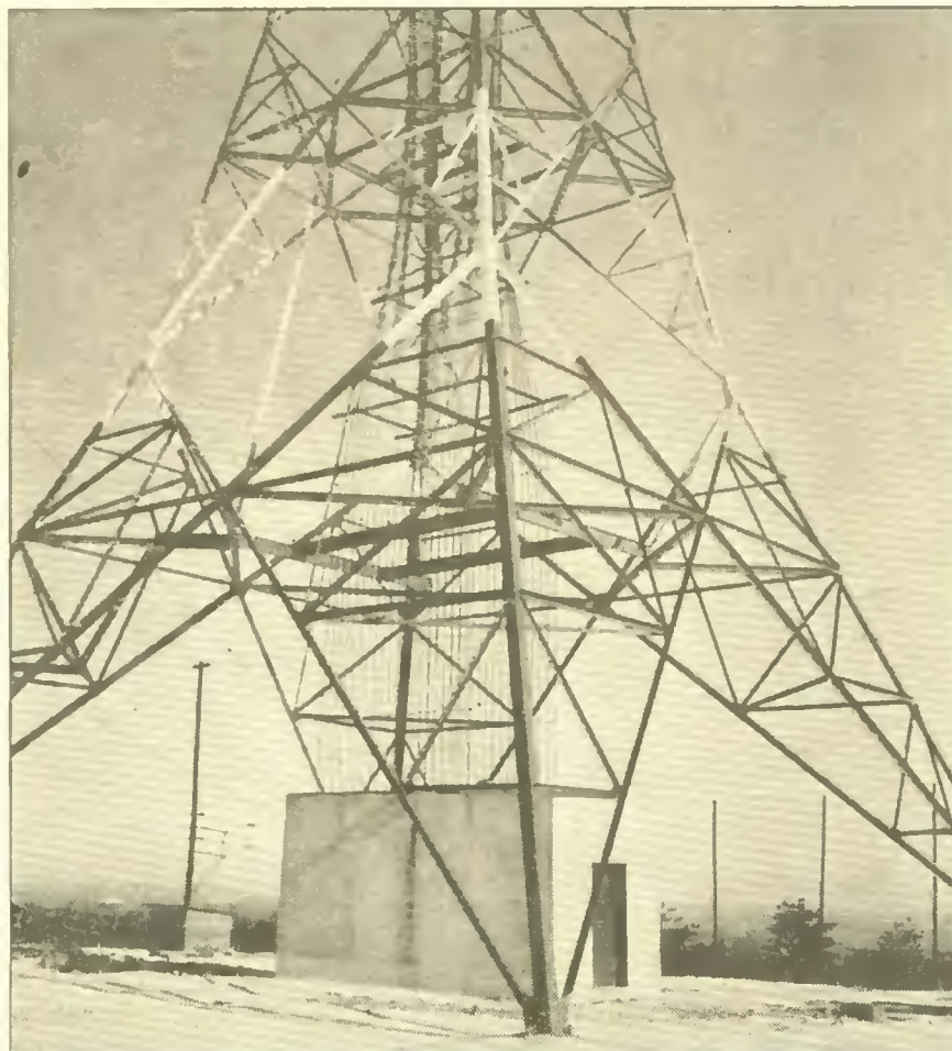
PLUMBER'S NIGHTMARE is an antenna tower like W43B's on Mount Asnebumskit in central Massachusetts. The lines radiating up the center of the structure's base are copper pipes that carry radio energy to ten sets of special FM antennas mounted on top of the 250-foot tower
